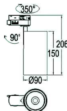
START 40 W
